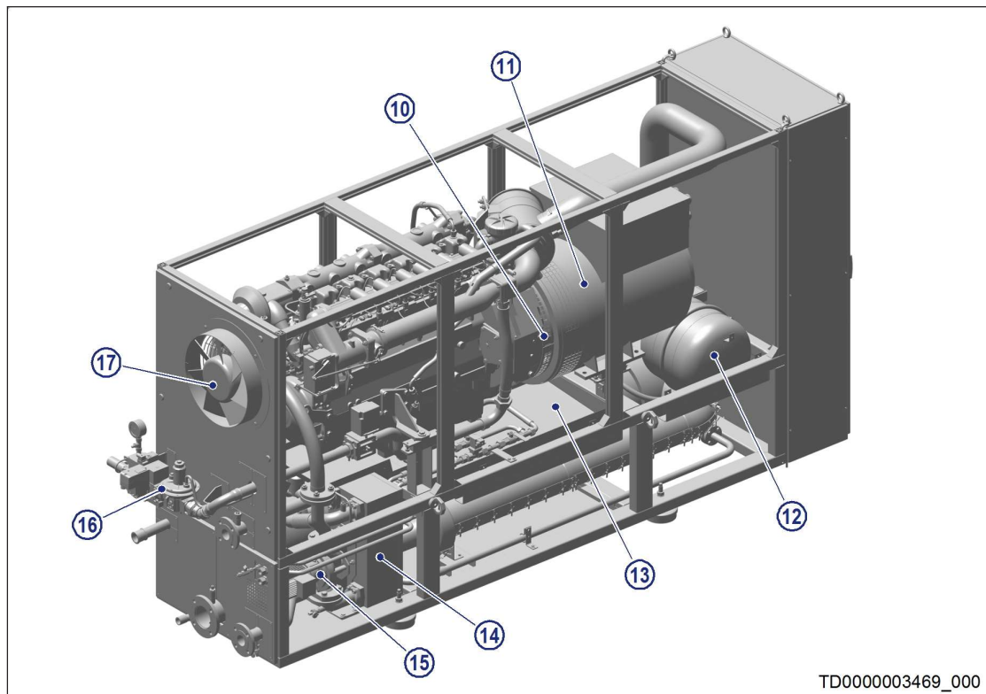
Figure 5: Module, engine side
